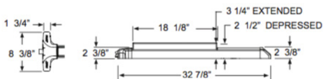
Device Dimensions
