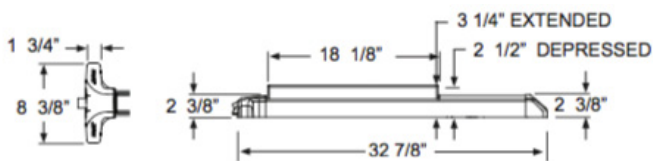
Device Dimensions
